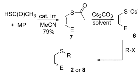
Scheme 3. Formation of cesium ( Z )-2-carbomethoxyethenethiolate and its general alkylation chemistry.
