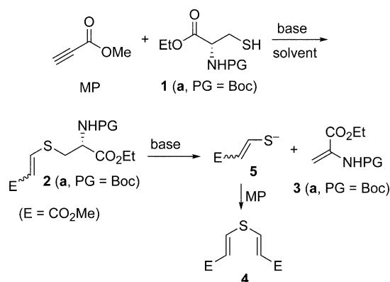
Scheme 1. The sensitivity of direct conjugate addition of MP with protected cysteines.
