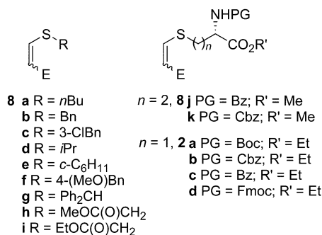
Figure 1. Alkylation products of cesium (Z)-2-carbomethoxyethenethiolate.
