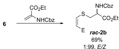
Scheme 4. Reaction of cesium (Z)-2-carbomethoxyethenethiolate with a dehydroalanine.
