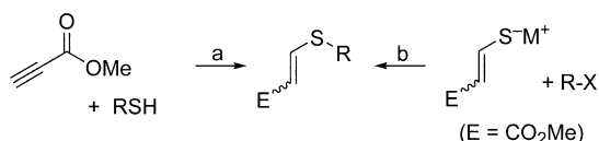
Scheme 2. Options for the preparation of 2-carboalkoxyethenyl thioethers.
